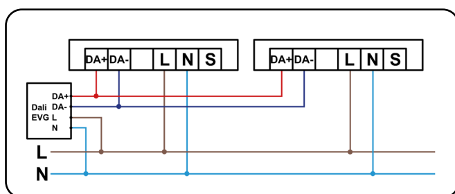
Master-Master-koppling Master-Master connection
