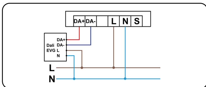
Master-Master-koppling Master-Master connection
